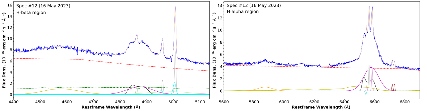
Fig. 6. Sample spectral decomposition in the H \beta (left) and H \alpha (right) regions for spectrum #12. In each panel, the blue solid line denotes the data, the total model is shown in beige, the solid black line denotes the Balmer diskline component, the solid magenta line denotes the broad Balmer Gaussian component, the red dashed line denotes the power-law component, and the dark green dashed line denotes the host galaxy emission. In the left panel (H \beta ), yellow, pale green, and pink respectively denote the F-, S-, and G-groups of Fe II emission, while the narrow Balmer and [O III] components are shown in gray, and the broad blueshifted [O III] components are shown in cyan. In the right panel (H \alpha ), He I emission is shown in orange, [S II] emission is shown in brown, [N II] emission is shown in pink, and the telluric atmospheric absorption feature is shown in cyan.
