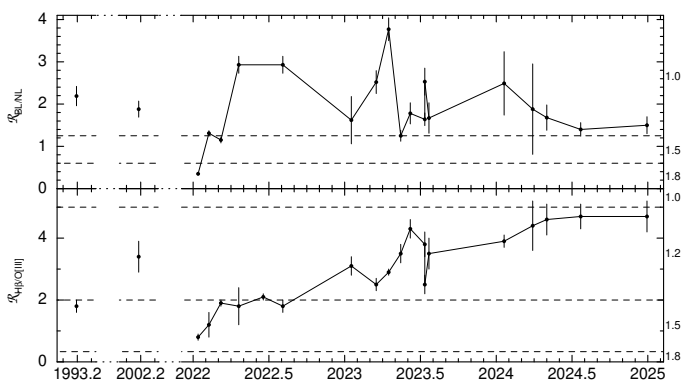
Fig. 9. R_{BL/NL} (top panel) and R_{H\beta/[O III]} (bottom panel) as a function of time. The horizontal dashed lines denote subtype classification boundaries following Runco et al. (2016, top panel) and Winkler (1992, bottom panel).
