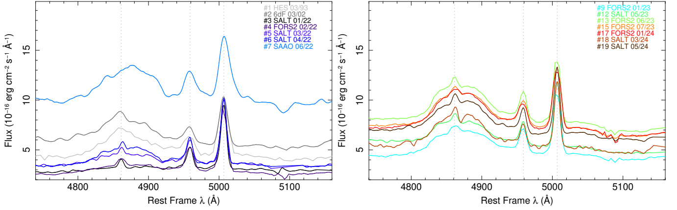
Fig. 5. H \beta and [O III] regions of selected optical spectra. The latter spectra (right panel) correspond to the resurgence of the diskline component, as discussed below. These spectra have been gray-scaled so that the integrated [O III] fluxes match. Smoothing has been applied for visual clarity only, using a boxcar of width 5 Å for all spectra, except for #2 and #7 where the width was 10 Å.
