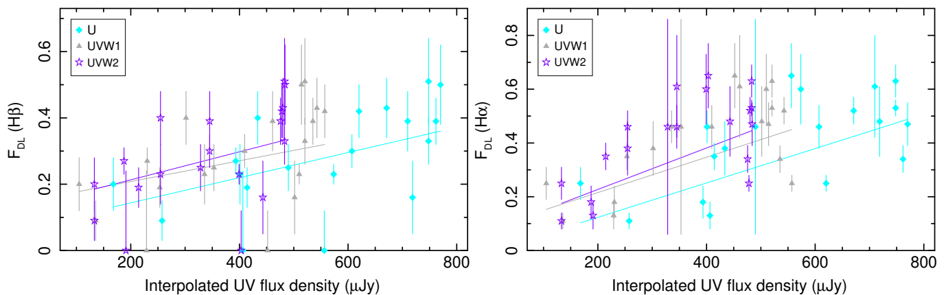
Fig. 8. F_{DL} , the ratio of diskline component intensity to total broad-line intensity for the H\beta line (left panel) and H\alpha line (right panel), as a function of UV flux density, interpolated to match the dates when the optical spectra were taken. Cyan, gray, and purple denote U, UVW1, and UVW2 flux densities, respectively. The solid lines indicate the best-fitting linear relations, meant to guide the eye. Positive correlations occur in all bands for both H\beta and H\alpha , indicating a link between UV continuum emission and the broad Balmer profiles.
