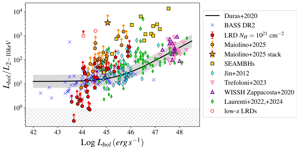
Fig. 5: X-ray bolometric correction, \kappa_{\text{bol,X}} = L_{\text{bol}}/L_{2-10\text{keV}} , as a function of L_{\text{bol}} . Shown are LRDs (Yue et al. 2024, red circles), JWST-selected AGN (Maiolino et al. 2025, orange circles), BASS AGN (Gupta et al. 2024, blue crosses), SEAMBHs (Tortosa et al. 2023, yellow squares) and NLS1s (Jin et al. 2012b, cyan diamonds). The orange star marks the stacked X-ray measurement of the non-detected sources from Maiolino et al. 2025. L_{\text{bol}} is derived from the broad H\alpha luminosity following Stern & Laor 2012, as in Maiolino et al. 2025. L_{\text{bol}} for BASS, SEAMBHs and NLS1 is from SED-fitting while for LRDs and JWST-selected AGN L_{\text{bol}} is derived from the broad H\alpha luminosity following Stern & Laor 2012, as in Maiolino et al. 2025. Also shown are low z LRDs analogues (Lin et al. 2026, red empty circles), hyper-luminous QSOs at z \sim 2 - 4 from the WISSH sample (Zappacosta et al. 2020, purple empty triangles), SDSS DR7 QSOs at z \approx 3.0 - 3.3 (Trefoloni et al. 2023, pink empty inverted triangle) and 0.4 < z < 3.3 radio-quiet highly accreting AGN (Laurenti et al. 2022, 2024, green diamonds). The black line indicates the relation from Duras et al. 2020, with the shaded region showing its 1\sigma uncertainty and the hatched region indicates the unphysical regime where \kappa_{\text{bol,X}} < 1 .
