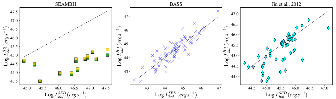
Fig. 4: Bolometric luminosity estimated from SED-fitting ( L_{\text{bol}}^{\text{SED}} ) vs bolometric luminosity derived from the broad H\alpha luminosity following Stern & Laor 2012 ( L_{\text{bol}}^{H\alpha} ). Left panel: we report L_{\text{bol}}^{H\alpha} using the observed L_{H\alpha} (green squares) and the extinction corrected one (yellow squares) for SEAMBHs; Central panel: the BASS AGN (blue crosses); Right panel: NLS1s galaxies from Jin et al. (2012b) (cyan diamonds). The black dashed line indicates the one-to-one relation in each panel.
