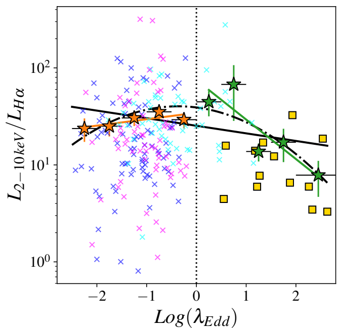
Fig. 3: The L_{2-10\text{keV}}/L_{\text{H}\alpha} - \lambda_{\text{Edd}} relation. We used the same colour code as Fig. 2. Solid black line is the best fitting linear relation considering the complete sample. We reported also the best fitting linear relation for the sub- (orange) and super- (green) Eddington sources. The stars represent the mean value in each \lambda_{\text{Edd}} bin and are shown for illustrative purposes only. Given the large intrinsic scatter (spanning \geq 2 orders of magnitude in L_{2-10\text{keV}}/L_{\text{H}\alpha} ), these averages are not used for \chi^2 minimization or quantitative inference. A quadratic fit (dotted-dashed curve) is shown to illustrate curvature in the trend. This figure includes only low-redshift AGN with joint detections in both X-rays and \text{H}\alpha ; no upper limits are included in this analysis.
