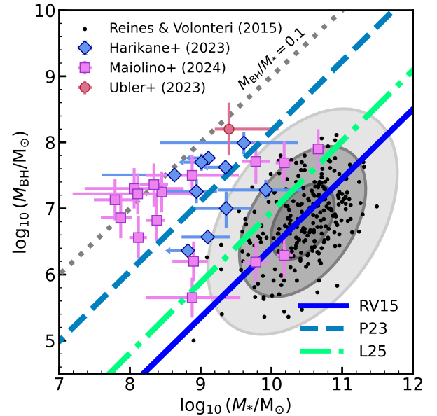
Figure 3. A comparison of the Reines & Volonteri (2015) , Pacucci et al. (2023) , and Li et al. (2025) M_{\text{BH}} - M_* relations with the local sample of AGN from Reines & Volonteri (2015) (black points) and the faint AGN samples of Maiolino et al. (2024) , Harikane et al. (2023) , and Übler et al. (2023) . The grey ellipses are the 1\sigma , 2\sigma , and 3\sigma confidence ellipses for the Reines & Volonteri (2015) sample.
