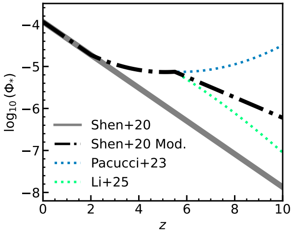
Figure 9. The evolution of the normalisation ( \Phi_{\star} ) at the break luminosity ( L_{\star} ) for the fiducial Shen et al. (2020) global fit A (grey solid line), our reference LF (black dot-dashed line), and the evolution necessary to match the estimates from the SMF with an initial redshift of z_i = 10 (dotted lines).
