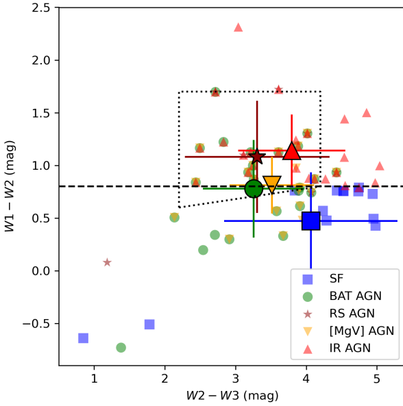
Fig. 2. WISE color-color diagram showing the five subsamples, as indicated by the symbols. The uncertainties are comparable to the symbol sizes. The large symbols with error bars correspond to the mean values for each subsample, with the error bars representing the standard deviation. The dashed line represents the threshold W1 - W2 = 0.8 , while the dotted polygon marks the region typically occupied by Seyfert galaxies (Jarrett et al. 2011).
