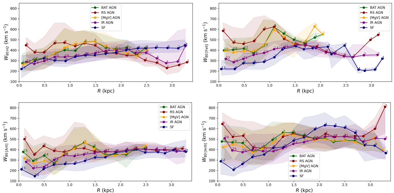
Fig. 5. Radial W_{80} profiles for H_2 (top left), [Fe\ II] (top right), [Ar\ II] (bottom left) and [Ar\ III] (bottom right) for the five subsamples, as indicated by the different colors. These profiles are computed as median values of W_{80} and distance of the spaxel from the position of the continuum peak, within circular rings of 250 pc width. The numbers next to each point indicate the number of galaxies used to compute it, and the shaded regions represent the range between the 25th and 75th percentiles of the W_{80} values within each radial bin, illustrating the spread of values observed in each emission line
