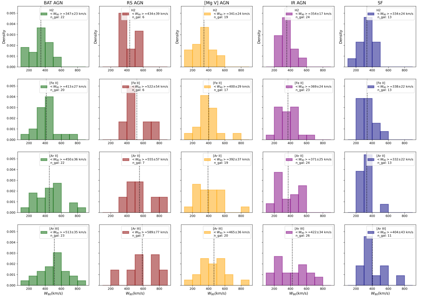
Fig. 4. Nuclear W_{80} values for the H_2 S(5), [Fe II], [Ar II], and [Ar III] emission lines — ordered by increasing ionization potential from top to bottom — are shown for the five subsamples, displayed in separate columns. The W_{80} values are estimated as the flux weighted mean W_{80} values of spaxels within a radius of 0.5 arcsec centred at the peak or the continuum emission. The mean values (indicated by vertical dashed lines), standard error
