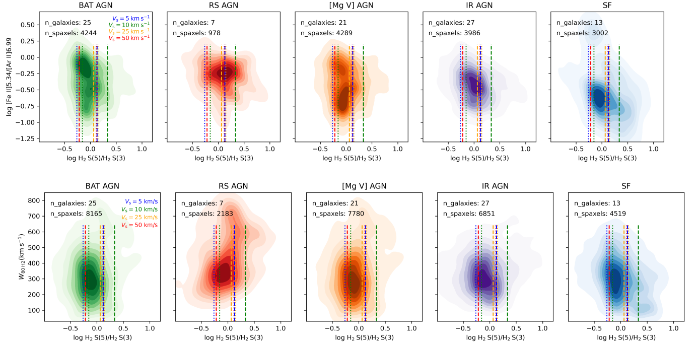
Fig. 8. Density plots for [\text{Fe II}]\lambda 5.3403\mu\text{m}/[\text{Ar II}]\lambda 6.9853\mu\text{m} vs. \text{H}_2 \text{S}(5)/\text{H}_2 \text{S}(3) (top) and W_{80} for the \text{H}_2 \text{S}(5) line vs. \text{H}_2 \text{S}(5)/\text{H}_2 \text{S}(3) (bottom) for all subsamples. The vertical lines represent mean \text{H}_2 \text{S}(5)/\text{H}_2 \text{S}(3) predictions of the shock models from Kristensen et al. (2023) for velocities of 5, 10, 25 and 50 \text{ km s}^{-1} (different colors) and densities of n_H = 10^3 (dotted lines) and n_H = 10^6 \text{ cm}^{-3} (dashed lines).
