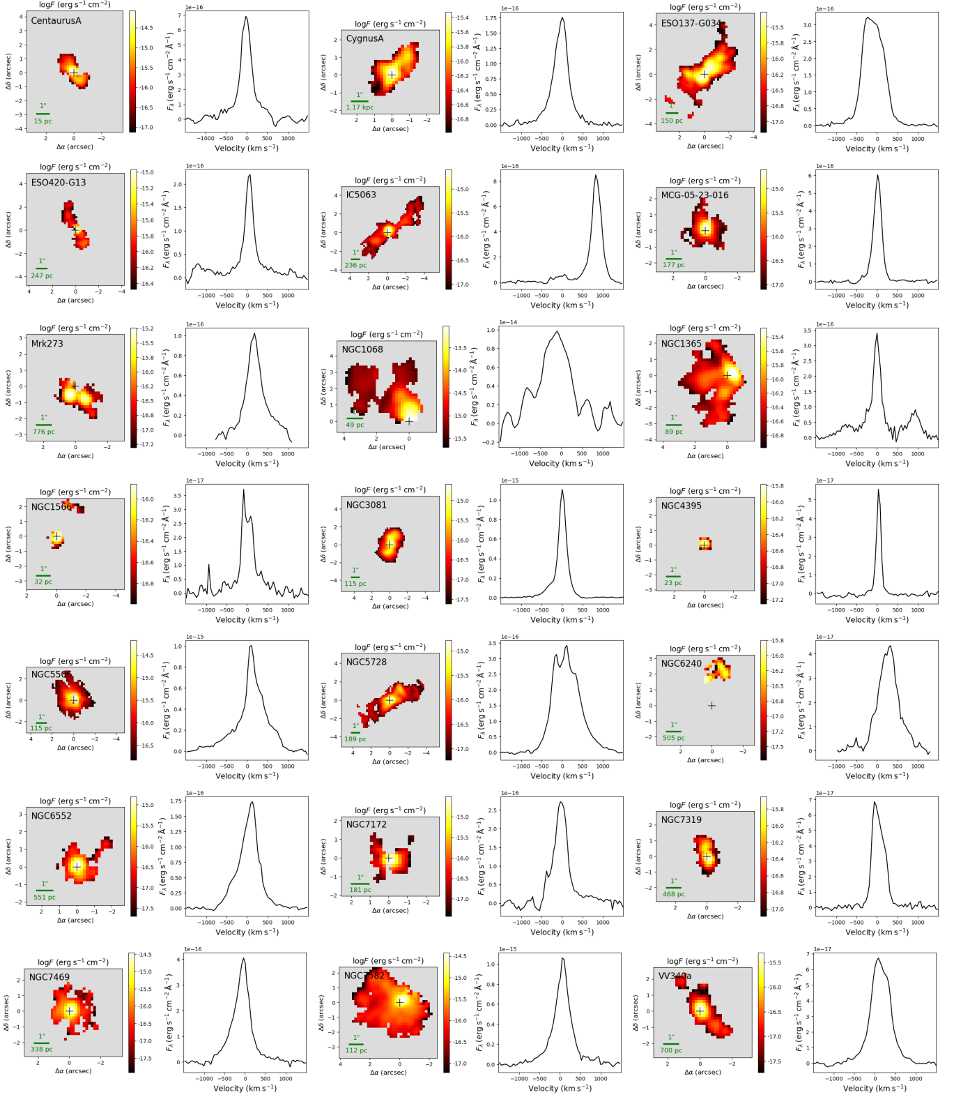
Fig. B.1. [\text{Mg v}]\lambda 5.6098\mu\text{m} flux distributions for galaxies with coronal line emission in our sample. The maps illustrate the flux distributions, with gray regions indicating areas where the corresponding emission line is not detected at \text{SNR} > 5 . The plots display the [\text{Mg v}]\lambda 5.6098\mu\text{m} integrated profiles, obtained by summing the observed profiles across all detected spaxels and subtracting the continuum. The name of each galaxy is shown in the top-left corner of each plot, the spatial scale is shown in the bottom-left corner, and the central cross marks the position of the galaxy's nucleus.
