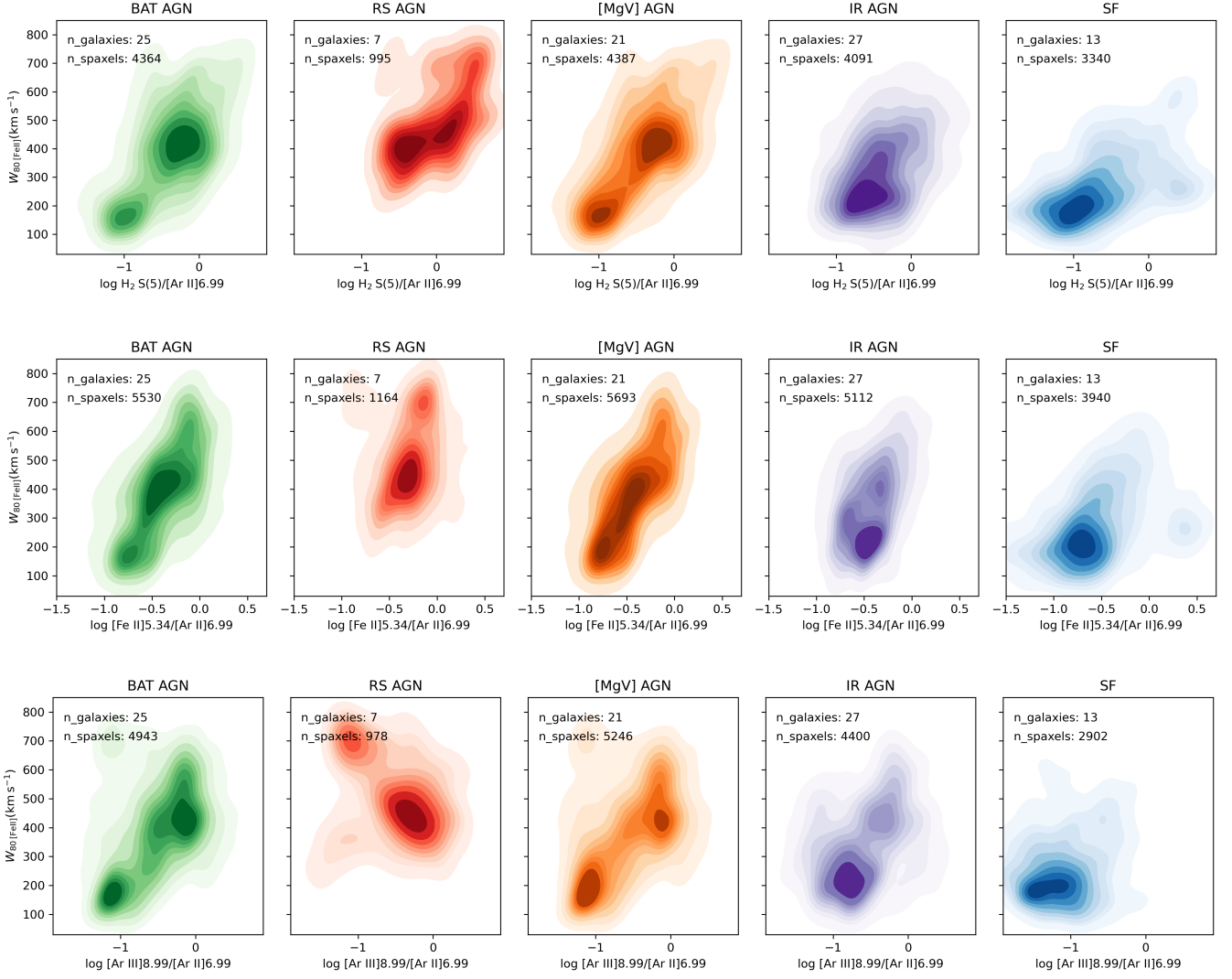
Fig. 6. Density maps of W_{80} for [\text{Fe II}]\lambda 5.3403\ \mu\text{m} emission line as a function of the flux ratios: \text{H}_2\text{ S}(5)\lambda 6.9091\ \mu\text{m}/[\text{Ar II}]\lambda 6.9853\ \mu\text{m} (top panels), [\text{Fe II}]\lambda 5.3403\ \mu\text{m}/[\text{Ar II}]\lambda 6.9853\ \mu\text{m} (middle panels), and [\text{Ar III}]\lambda 8.9914\ \mu\text{m}/[\text{Ar II}]\lambda 6.9853\ \mu\text{m} (bottom panels). The contours are spaced at intervals of 10% in data density. Results are shown for the different subsamples, as identified in the title of each panel.
