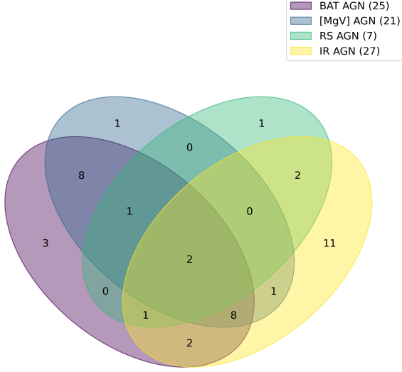
Fig. 1. Venn diagram illustrating the overlap among the different AGN subsamples.
