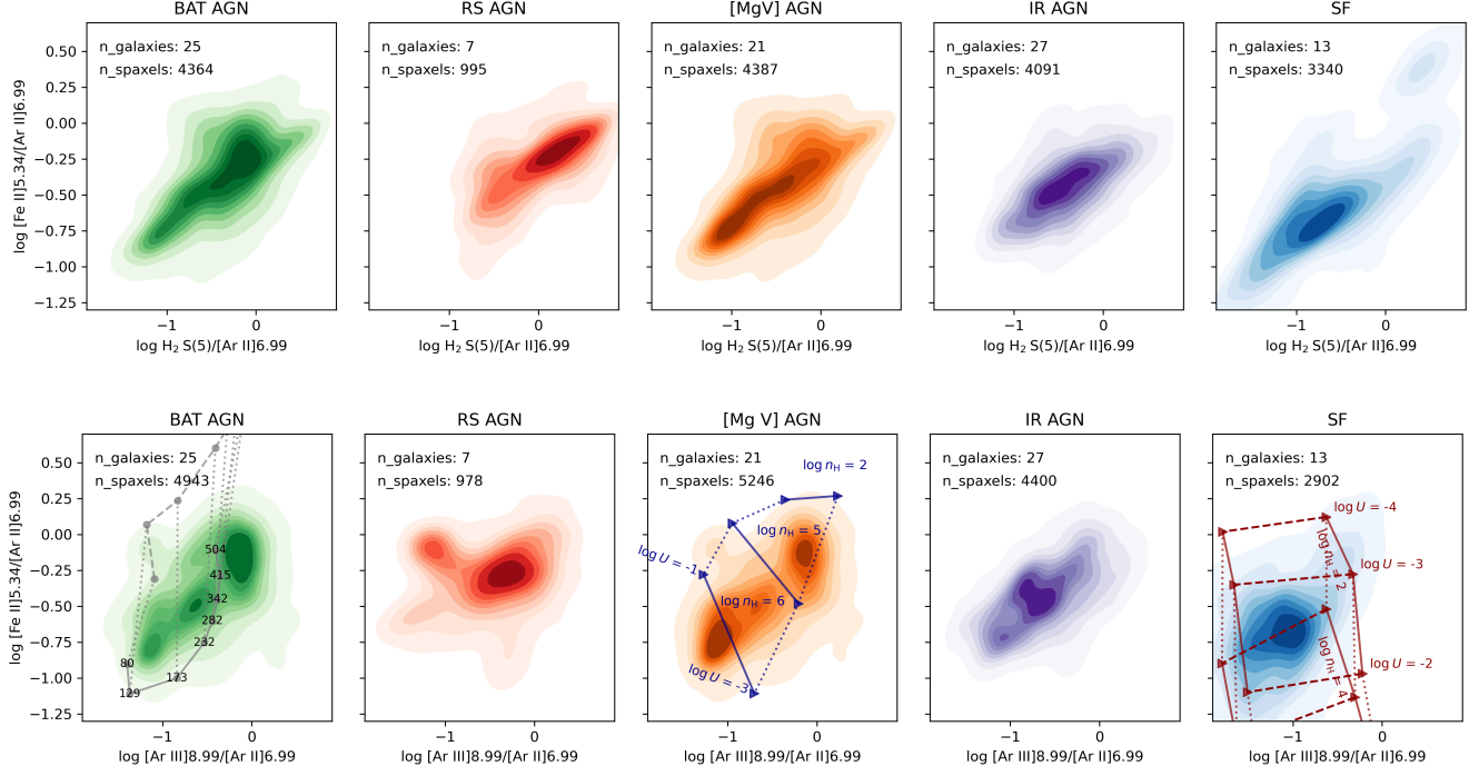
Fig. 7. Density plots for the [\text{Fe II}]\lambda 5.3403\mu\text{m}/[\text{Ar II}]\lambda 6.9853\mu\text{m} vs. \text{H}_2 \text{S}(5)/[\text{Ar II}]\lambda 6.9853\mu\text{m} (top panels) and [\text{Fe II}]\lambda 5.3403\mu\text{m}/[\text{Ar II}]\lambda 6.9853\mu\text{m} vs. [\text{Ar III}]\lambda 8.9914\mu\text{m}/[\text{Ar II}]\lambda 6.9853\mu\text{m} (bottom panels). The dark red lines (bottom-right panel) show predictions from photoionization models of star-forming regions, assuming stellar clusters aged 6 and 7 Myr. Solid lines indicate different gas densities, dotted lines correspond to varying ionization parameters (as labeled in the figure), and the predictions for both cluster ages are connected by dashed lines. Similarly, results from AGN photoionization models are shown as dark blue lines (bottom-central panel). The gray lines and filled circles (bottom-left panel) are predictions of fast shock models from Pereira-Santaella et al. (2024) using the MAPPINGS v code ( Sutherland & Dopita 2017 ) for \log R_p = 6 (dashed) and \log R_p = 8 (continuous). The numbers indicate the shock velocities in \text{km s}^{-1} .
