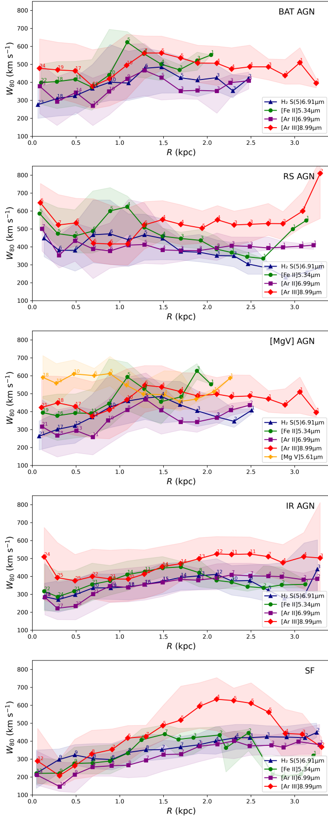
Fig. C.1. The W_{80} radial profiles for the four emission lines are presented for the BAT AGN, RS AGN, [Mg v] AGN, IR AGN and SF subsamples, from top to bottom, respectively. These profiles were computed following the same methodology as those shown in Fig. 5.
