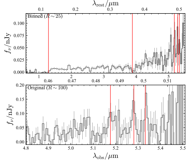
Figure 9. Spectrum of JADES-67592 ( z_{\text{spec}} = 9.65 ) downloaded from DJA. The upper and lower panels show the overall four times binned PRISM spectra ( R \sim 25 ) and the zoom-in original ( R \sim 100 ) spectra around H \beta + [O III] \lambda\lambda 4959, 5007 . The wavelengths of Ly \alpha , Balmer limit, H \beta , and [O III] \lambda\lambda 4959, 5007 are shown in red vertical lines.
