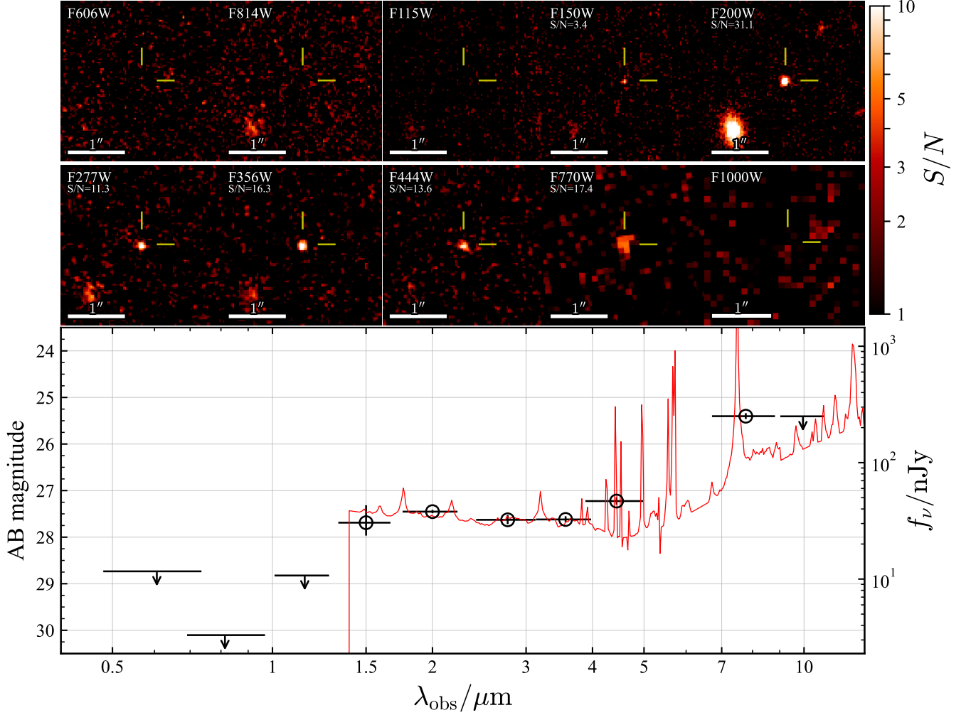
Figure 3. (Upper) HST + JWST 3'' \times 3'' cutout images centered on CW-LRD-z10. Each image is scaled by a noise map. If detected, the S/N measured from forced photometry is shown in the top left corner. (Lower) Observed SED of CW-LRD-z10. For F606W, F814W, F115W, F1000W, and F2100W, we plot the 2\sigma upper limits. The red line indicates the best-fit LRD model SED from the SED fitting analysis (Section 4.2)
