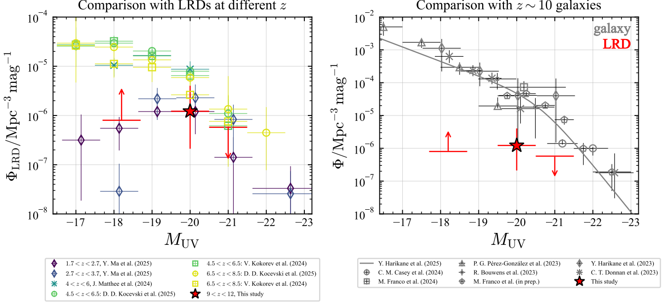
Figure 6. Luminosity function of z \sim 10 LRDs shown by the red star data point. (Left) Comparison with the luminosity functions of LRDs at lower redshifts ( 1.7 < z < 8.5 ) from previous studies (Y. Ma et al. 2025b; J. Matthee et al. 2024; D. D. Kocevski et al. 2025; V. Kokorev et al. 2024a). Note that the lower limit at M_{\text{UV}} = -18.2 and 9 < z < 12 is based on the assumption that only CAPERS-LRD-z9 (A. J. Taylor et al. 2025b) is a true z \sim 10 LRD in the selection by D. D. Kocevski et al. (2025), independently identified of the selection in this study. (Right) Comparison of the LRD luminosity function with that of galaxies at z \sim 10 (C. T. Donnan et al. 2023; Y. Harikane et al. 2023b; M. Franco et al. 2024; C. M. Casey et al. 2024; R. Bouwens et al. 2023; P. G. Pérez-González et al. 2023; M. Fracco et al. in prep.). Best-fit double power law model from Y. Harikane et al. (2025) is indicated by the black line.
