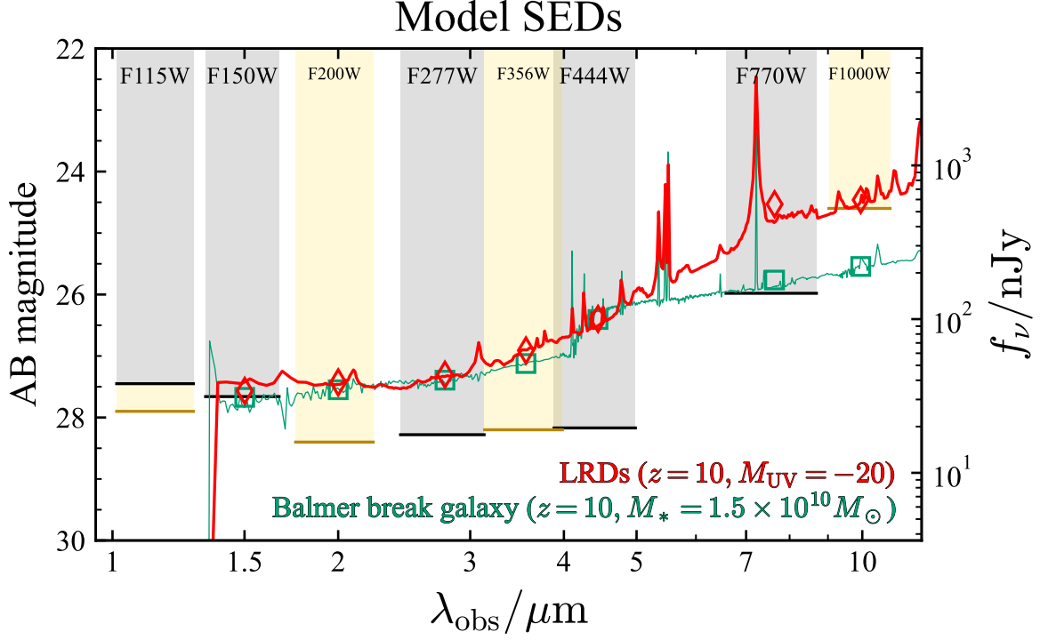
Figure 1. Model SED of a z = 10 LRD with M_{UV} = -20 (red) and 5\sigma depth for point sources in COSMOS-Web (F115W, F150W, F277W, F444W, and F770W) from C. M. Casey et al. (2023) and in COSMOS-3D (F115W, F200W, F356W, and F1000W) shown in gray and gold rectangles, respectively. Model SEDs of potential contaminants of the z \sim 10 LRD photometric selection, a z = 10 galaxy with a stellar-origin Balmer break with A_V = 0.5 and M_* = 1.5 \times 10^{10} M_\odot , is overlaid. The LRD model SED is from H. B. Akins et al. (2024), and the galaxy SED is generated using FSPS (C. Conroy et al. 2009; C. Conroy & J. E. Gunn 2010). The predicted model photometry is shown with diamonds for the LRD and squares for the galaxy. MIRI photometry is essential to distinguish between z \sim 10 LRDs and z \sim 10 galaxies with stellar-origin Balmer break.
