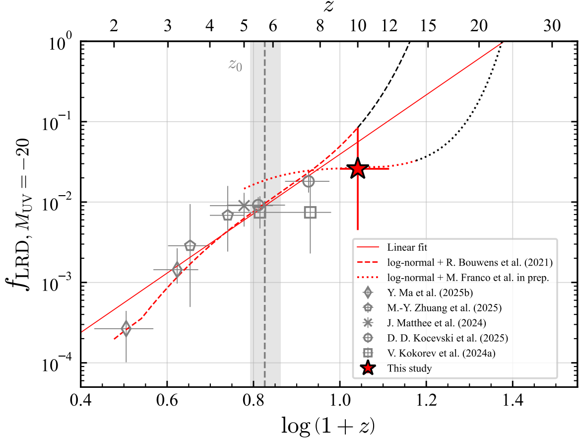
Figure 8. Redshift evolution of the LRD fraction relative to the overall galaxy population at M_{\text{UV}} = -20 . Symbols for lower-redshift LRDs (Y. Ma et al. 2025b; M.-Y. Zhuang et al. 2025; J. Matthee et al. 2024; D. D. Kocevski et al. 2025; V. Kokorev et al. 2024a) are the same as Figure 6 (left). The red solid line shows the best-fit linear model. The red dashed and dotted lines indicate the modeled f_{\text{LRD}} redshift evolution that combines the evolutions of the UV luminosity function of LRDs (the fitted log-normal distribution shown in Figure 7) and galaxies from R. J. Bouwens et al. (2021) and M. Franco et al. (in prep.), respectively. For each model, the black line indicates the extrapolation of each luminosity function evolution beyond the range constrained by observational data. The gray dashed line and shaded region indicate the fitted peak redshift of the log-normal distribution ( z_0 ).
