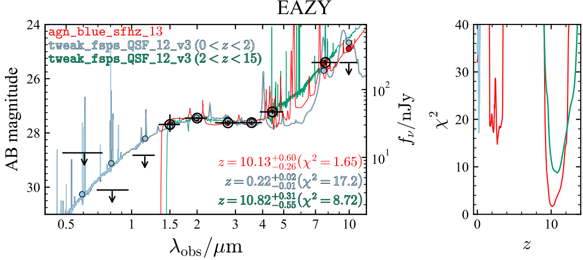
Figure 12. Same as Figure 4 but for the results with EAZY. Red, cyan, and green correspond to fits using the sorted_agn_blue_sfHz_13 template over 0 < z < 15 , the tweak_fsps_QSF_12_v3 template over 0 < z < 2 , and the tweak_fsps_QSF_12_v3 template over 2 < z < 15 , respectively.
