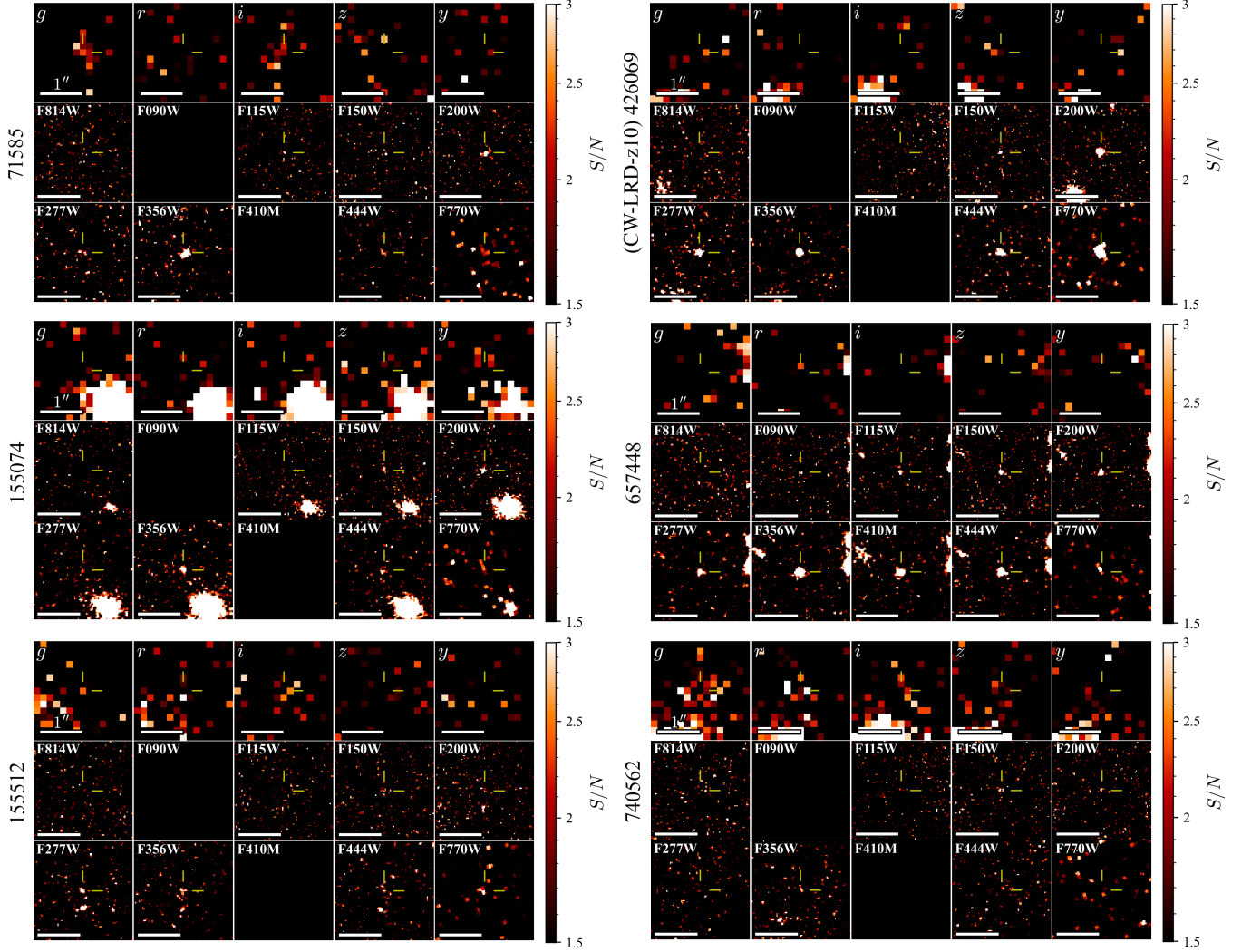
Figure 10. HSC ( grizy ), HST (F814W), and JWST 2''.5 \times 2''.5 cutout images centered on each object excluded in visual inspection. For comparison, we also plot CW-LRD-z10 (ID:426069). Each image is scaled by a noise map.
