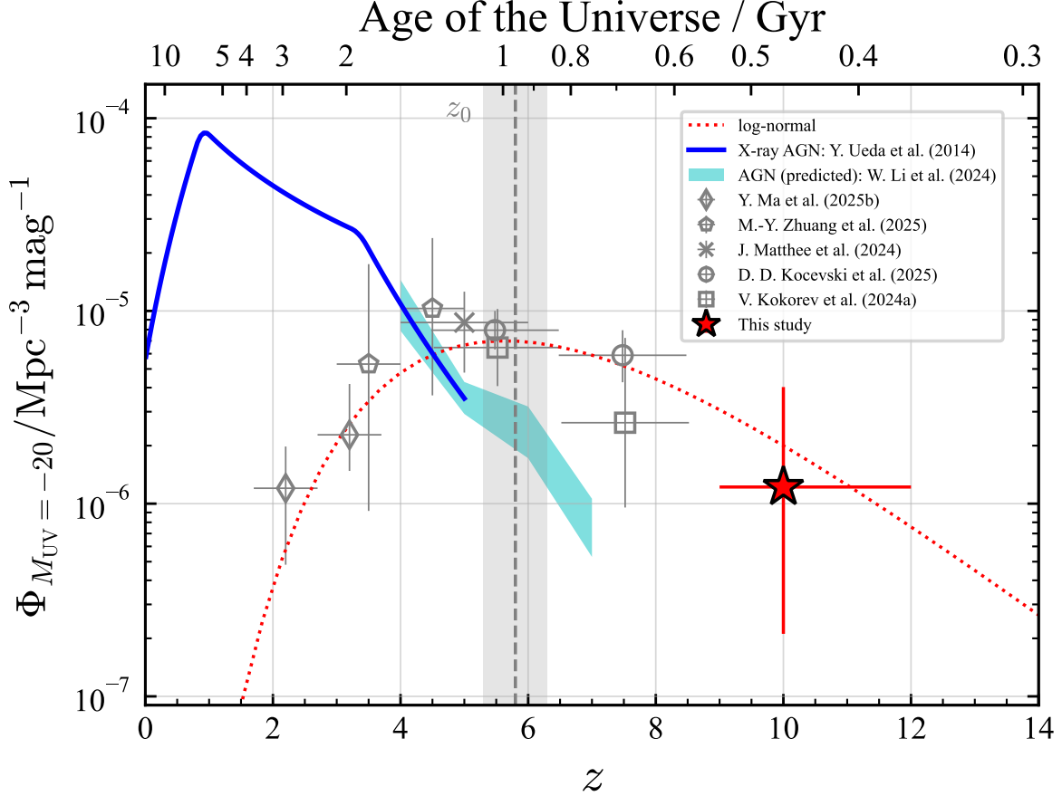
Figure 7. Redshift evolution of the luminosity function at M_{UV} = -20 . Symbols for lower-redshift LRDs (Y. Ma et al. 2025b; M.-Y. Zhuang et al. 2025; J. Matthee et al. 2024; D. D. Kocevski et al. 2025; V. Kokorev et al. 2024a) are the same as Figure 6 (left). The red dotted line indicates the best-fit log-normal distribution. The gray dashed line and shaded region indicate the best-fit peak redshift ( z_0 ). Blue line and cyan shaded region indicate the AGN luminosity function at M_{UV} = -20 from the X-rays (Y. Ueda et al. 2014) and model prediction (W. Li et al. 2024). Note that we assume an X-ray–UV luminosity ratio (E. Lusso & G. Risaliti 2016) and a photon index of \Gamma = 1.9 to convert the X-ray (Y. Ueda et al. 2014) to UV luminosity function.
