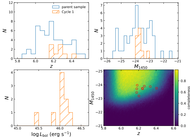
Figure 1. Properties of the Cycle 1 sample as drawn from SHELLQs (Matsuoka et al. 2018a): redshift, absolute UV magnitude, bolometric luminosity, and selection completeness as a function of absolute magnitude and redshift.
