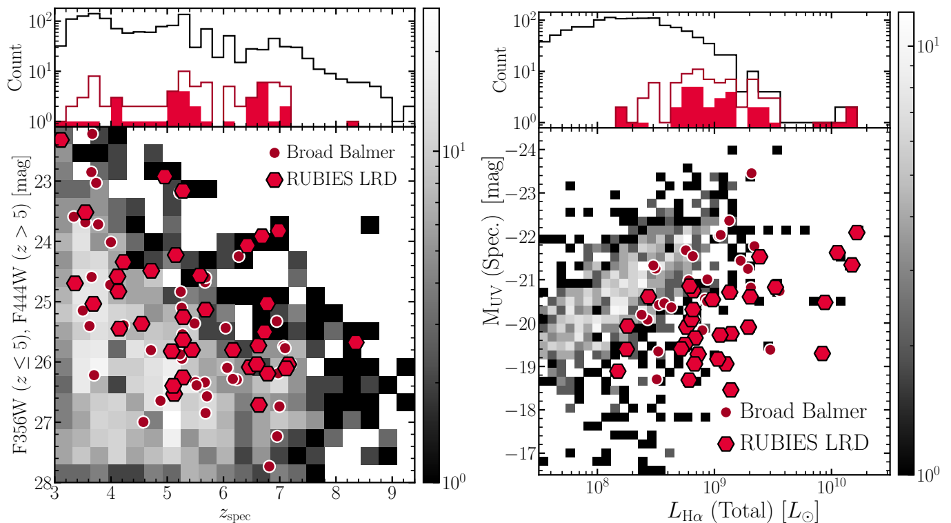
Fig. 8: Redshift vs. NIRCcam F356W (for z_{\text{spec}} \leq 5 ) or F444W (for z_{\text{spec}} > 5 ) is shown on the left, and absolute UV magnitude ( M_{\text{UV}} ) at 1500\text{\AA} , derived from rest-UV spectroscopic slopes, is plotted against total H\alpha luminosity on the right. RUBIES with robust z_{\text{spec}} > 3.1 are shown as a grey histogram. Broad-line sources are indicated with dark red circles, and LRDs, defined as galaxies with v-shaped continua, broad Balmer lines, and dominant rest-optical point sources, are shown as light red hexagons. At fixed L_{H\alpha} LRDs are faint in the rest-UV compared to the full population. Conversely, extreme H\alpha emitters ( L_{H\alpha} \gtrsim 10^{10} M_{\odot} ) are dominated by LRDs, i.e. LRDs constitute the most luminous H\alpha emitters at fixed UV luminosity.
