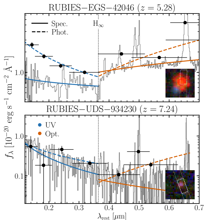
Fig. 3: Rest-UV (blue) and rest-optical (orange) continuum fitting of RUBIES-EGS-42046 (top) and RUBIES-UDS-934230 (bottom) from PRISM spectroscopy (solid) and NIRCcam photometry (dashed). We inset 0.5'' \times 0.5'' NIRCcam F444W/F277W/F150W RGB cutouts of the sources as well. We emphasize that spectroscopic rest-optical continuum fitting can mitigate the effect of strong emission lines but can suffer in S/N in the rest-UV where the spectrum is fainter or cannot capture extended rest-UV emission due to slit losses.
