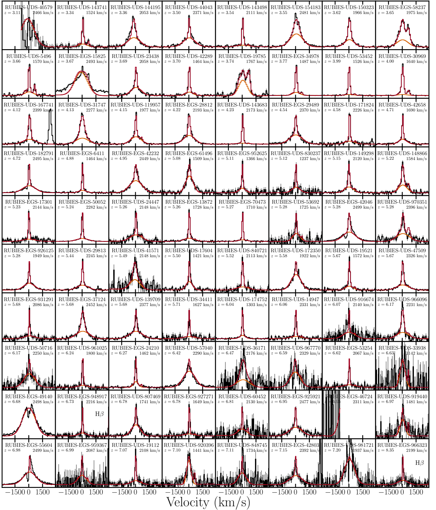
Fig. B.2: All robust Broad-Balmer line objects found in the RUBIES data, organized by redshift. We plot the linear-scaled G395M \pm 3000 \text{ km s}^{-1} zoom-in of the H\alpha line where available, otherwise H\beta , with the broad component fit superimposed in red and the broad Balmer component in orange. We also include text containing the FWHM of the broad component as well.
