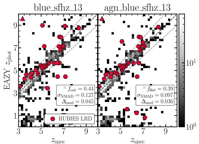
Fig. 10: Best-fit photometric versus spectroscopic redshift for RUBIES sources with robust z_{\text{spec}} > 3.1 (grey histogram) and the LRD sample (red hexagons; triangle indicates outlier of plot). Photometric redshifts were measured using eazy ( Brammer et al. 2008 ) with two different template sets: the blue_sfhz_13 set optimized for high-redshift galaxies (left) and the agn_blue_sfhz_13 set which additionally includes an AGN template constructed from the LRD of Killi et al. (2024) and a torus model (right). Dashed lines show |\Delta z|/(1 + z_{\text{spec}}) = 0.1 . Although including this AGN template reduces the number of outliers and photometric redshift scatter for the LRD sample, a small bias toward higher photometric redshifts remains.
