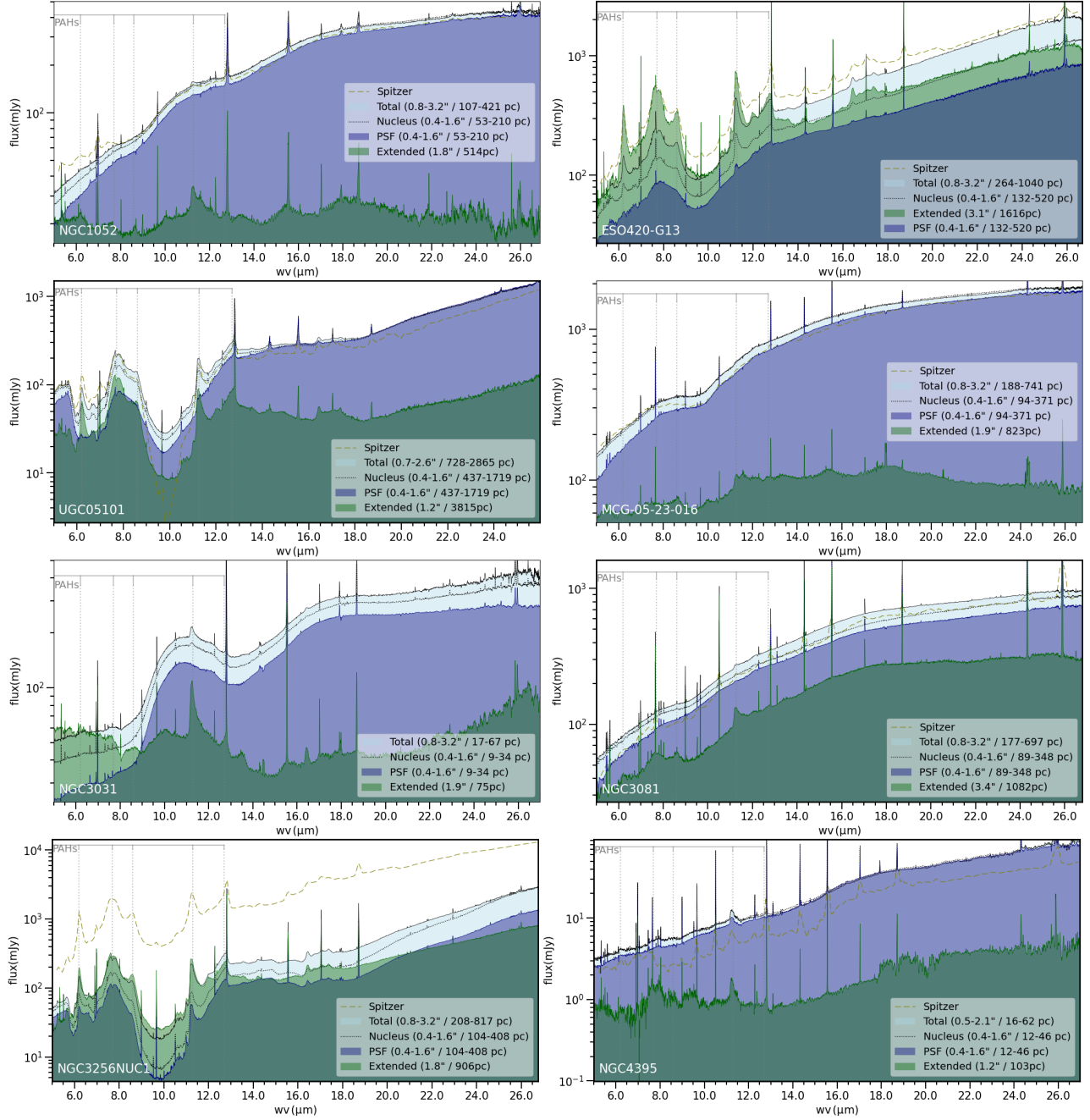
Figure B1. Each panel shows the total (solid-black line filled in light blue), nuclear (dotted-black line), PSF (solid-blue line filled in blue), and circumnuclear (solid-green line filled in green) spectra. When available, Spitzer /IRS spectrum is shown with the long-dashed green line. Legends show the spatial scales for each spectral extraction radius.
