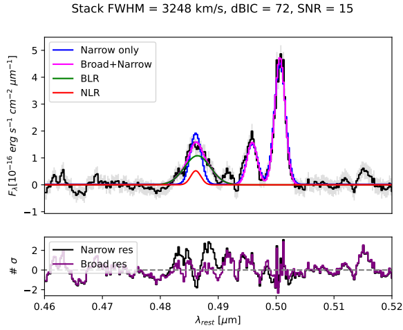
Figure B2. Stacked, continuum subtracted spectrum of the four objects visually identified to have broad H\beta in prism. The plot is organized the same as the individual ones in Figure B1 . It can be seen that not including a broad line in the fit leaves significant symmetric wings in the residual. In addition, the narrow-line fit would result in a [O\text{III}]/H\beta ratio of 3, uncharacteristically low for these high-redshift objects.
