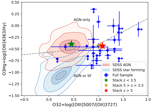
Figure 14. Diagnostic diagram of the [\text{O III}]\lambda 4363/\text{H}\gamma and [\text{O III}]\lambda 5007/[\text{O II}]\lambda 3727 from Mazzolari et al. (2024c) . The AGN and star forming galaxies from SDSS are shown in red and blue contours respectively. Our sample sources and stacks are shown with blue circles and colored stars as in Figure 13 . The grey dashed line indicates the boundary between the region populated by AGN only (above it) and the one with a mixture of AGN and star forming galaxies (below it).
