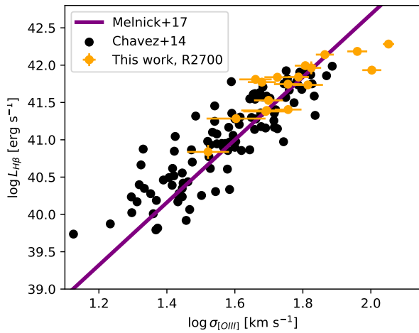
Figure 7. The H\beta luminosity - [O III] velocity dispersion relationship. The purple line shows the empirical relationship of Melnick et al. (2017) while emission line galaxy measurements by Chávez et al. (2014) are shown by black dots. Our Type 1 AGN with R2700 data available are shown with yellow points. The Type 1 AGN are all consistent with the standard relation.
