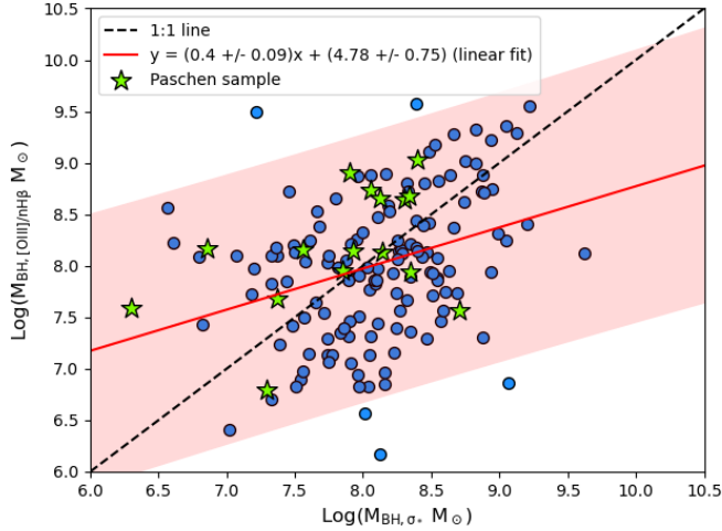
Figure 5. Left: Comparison of L_{[\text{O III}]} / L_{\text{nH}\beta} -derived black hole masses ( M_{\text{BH},[\text{O III}]/\text{nH}\beta} ) and those calculated from the host stellar velocity dispersion ( M_{\text{BH},\sigma^*} ). For reference, the AGN we used to assess the agreement between M_{\text{BH},[\text{O III}]/\text{nH}\beta} and the Paschen-derived black hole masses are shown by the green stars. On average, the values are consistent to within 0.08 dex, albeit with a wide scatter ( 0.74 dex). Line styles are the same as Figure 1.
