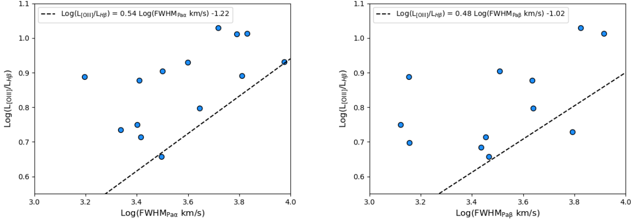
Figure 2. Comparison of narrow line region ionization field hardness ( \log(L_{\text{[O III]}}/L_{\text{H}\beta}) ) and broad line region kinematics traced by the FWHM of the broad \text{Pa}\alpha (left) and \text{Pa}\beta (right) lines. We find a significant correlation between NLR ionization field hardness and \text{FWHM}_{\text{Pa}\alpha} ( p -value = 0.0297) but an insignificant correlation with \text{FWHM}_{\text{Pa}\beta} ( p -value=0.0918). For reference, the expected relationship between \log(L_{\text{[O III]}}/L_{\text{H}\beta}) and \log(\text{FWHM}_{\text{Pa}\alpha}) and \log(\text{FWHM}_{\text{Pa}\beta}) , combining the results of Kim et al. (2010) and BM19 (Eqs. 9 and 10), is shown by the dashed black line. The correlation between ionization field hardness and BLR kinematics is weaker than that reported in BM19. Either such trends are only prominent when considering aggregate AGN spectra (as in BM19) and not individual measurements, the coupling between the NLR ionization field and the more distant BLR in which the Paschen lines form is weaker, or extinction in the BLR that extinguishes broad \text{H}\alpha in these AGN also depresses the Paschen emission relative to the unobscured AGN studied in BM19. Error bars are not shown here since they are generally smaller than the size of the symbols.
