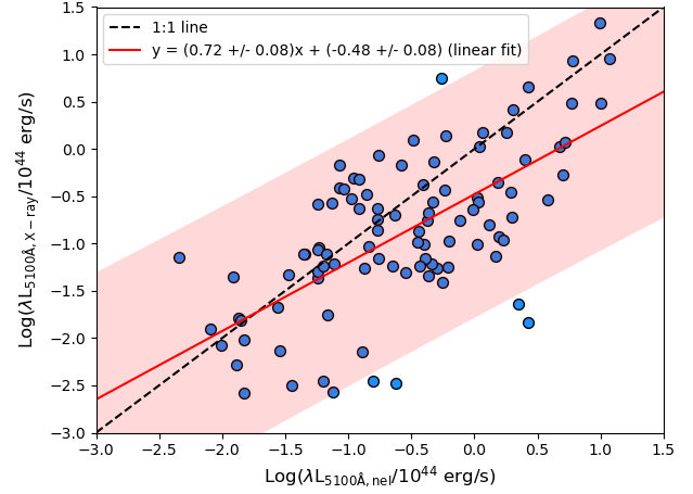
Figure 1. Comparison of estimates of the accretion disk luminosity at 5100 Å ( \lambda L_{5100\text{\AA}} ) using optical narrow emission lines ( \lambda L_{5100\text{\AA},\text{nel}} ) and the intrinsic 2-10 keV luminosity ( \lambda L_{5100\text{\AA},\text{X-ray}} ) as proxies. The black dashed line indicates the one-to-one relation, the red solid line is a linear fit to the data, and the shaded red region shows the 95% prediction interval for the linear fit. The mean offset (i.e., \log(\lambda L_{5100\text{\AA},\text{X-ray}}) - \log(\lambda L_{5100\text{\AA},\text{nel}}) ) is -0.32 \pm 0.68 dex. While these quantities are statistically equal, this scatter of \sim 5 in \lambda L_{5100\text{\AA}} can propagate to uncertainties of \sim 2 in black hole mass estimates when using Equation 1. Error bars are not shown here since they are generally smaller than the size of the symbols.
