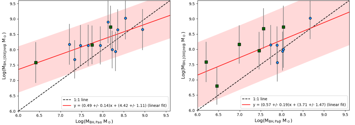
Figure 3. Comparison of black hole masses calculated using the L_{[\text{O III}]} / L_{\text{nH}\beta} method in Equation 1 ( M_{\text{BH},[\text{O III}]/\text{nH}\beta} ) and those derived from the broad Pa \alpha line (left) and broad Pa \beta line (right). The dark green squares indicate AGN whose Paschen emission line parameters were derived from the den Brok et al. (2022) catalog where the quality of the spectral fit is not reported. M_{\text{BH},[\text{O III}]/\text{nH}\beta} is systematically larger than masses derived via the broad Paschen lines by a factor of \sim 2-3 , though the scatter is slightly larger than these offsets (see Table 4). The agreements between the Paschen-derived black hole masses and those from the L_{[\text{O III}]} / L_{\text{nH}\beta} method is better when censoring the den Brok et al. (2022) data (with mean offsets of 0.30 \pm 0.42 dex and 0.09 \pm 0.26 dex when comparing M_{\text{BH},[\text{O III}]/\text{nH}\beta} with M_{\text{BH},\text{Pa}\alpha} and M_{\text{BH},\text{Pa}\beta} , respectively), but small number statistics preclude us from drawing conclusions from this censored dataset. Error bars are derived by propagating the 0.68 dex uncertainty on \lambda L_{5100\text{\AA}} and the uncertainties on \text{FWHM}_{\text{bH}\alpha} (from the errors on the slope and normalization in Equation 2) to the M_{\text{BH},[\text{O III}]/\text{nH}\beta} equation (Equation 1).
